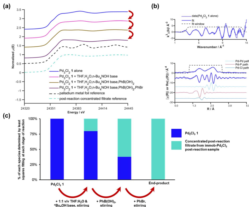
Fig. 9 Pd K-edge XANES spectra of the Pd 3 Cl 2 cluster 1 alone (blue), and after stepwise addition of H 2 O/THF and n Bu 4 NOH base (pink), phenylboronic acid (brown), and phenyl bromide (platinium purple) (a); Pd K-edge k -space and R -space EXAFS data and fits of the initial Pd 3 Cl 2 cluster 1, dashed blue lines denote the data, solid blue lines show the fit, with the fitting window shown above and the contributing paths from Pd–Pd, Pd–P and Pd–Cl shown below (b); plot of the contributions determined by least squares fitting the spectra shown in (a) for the stepwise reaction of the initial Pd 3 Cl 2 cluster 1 and the concentrated post reaction filtrate from the immob-Pd 3 Cl 2 experiments as explained in the text (c). Spectra offset for clarity, the lowest XANES spectrum is correctly placed on the y-axis with all XANES spectra normalized between 0 and 1 and EXAFS oscillations centered around y = 0 prior to any offset.
