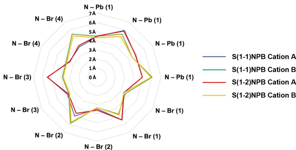
Fig. 7 (a) Schematic of cation A and B in S(1-1)NPB and S(1-2)NPB for calculation of N–Pb/Br distances (Tables S7 and S8†). Blue, red, black, and turquoise spheres denote Pb, Br, C, and N atoms, respectively. The obtained data for S(1-1)NPB is derived from our previously published work. 45 (b) Radar chart of the N–Pb/Br distances of type A and B cations in S(1-1)NPB and S(1-2)NPB. Blue and green lines denote the cation A and B of S(1-1)NPB, respectively. Red and yellow lines indicate the cation A and B of S(1-2)NPB, respectively.
