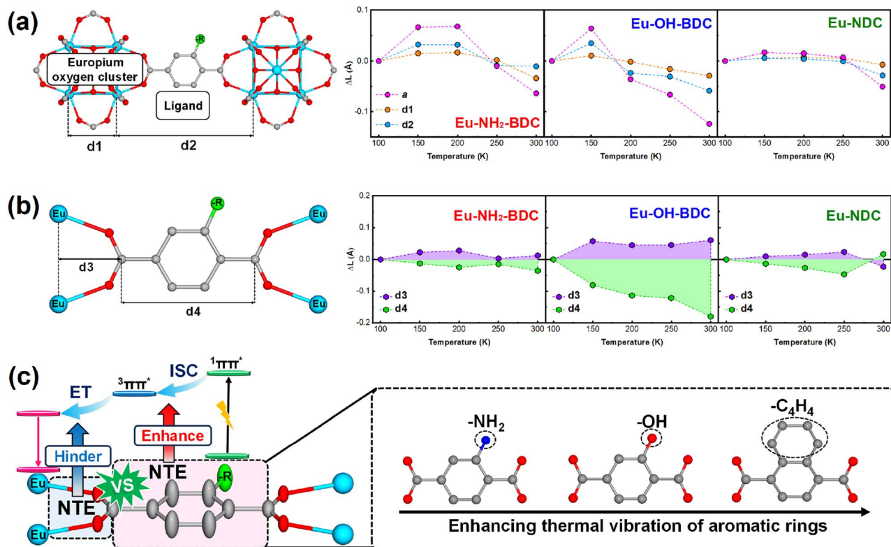
Fig. 4 NTE and luminescence thermal enhancement. The structure variation with temperature was obtained from VT-SCXRD. (a) Temperature dependent length changes of unit cell ( a ), europium oxygen cluster ( d1 ) and ligand ( d2 ) in Eu-NH 2 -BDC, Eu-OH-BDC, and Eu-NDC. (b) Temperature dependent horizontal length of carboxylic acids ( d3 ) and aromatic rings ( d4 ) in Eu-NH 2 -BDC, Eu-OH-BDC, and Eu-NDC. (c) Schematic mechanism of functional group modifications affecting luminescence thermal enhancement.
