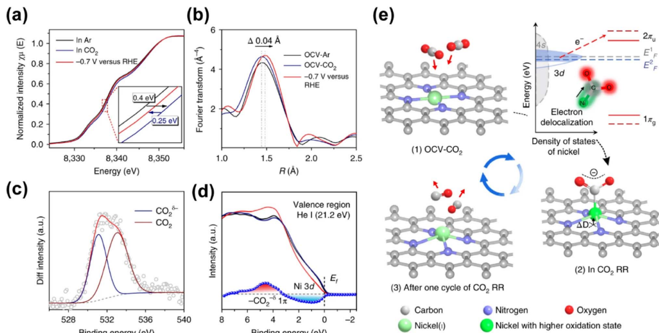
Fig. 15 (a) Normalized operando Ni K-edge XANES spectra for A-Ni-NG at various biases ( versus RHE) in 0.5 M \text{KHCO}_3 aqueous solution at room temperature and 1 atm of Ar or \text{CO}_2 . The inset shows the enlarged Ni K-edge XANES spectra. (b) Fourier transform magnitudes of EXAFS spectra (without phase correction) of A-Ni-NG under open-circuit voltage bias in Ar (OCV-Ar) and \text{CO}_2 (OCV- \text{CO}_2 ), and at -0.7 V ( versus RHE), in which an expanded Ni-N bond was detected. (c) Change in the XPS O 1s intensity induced by \text{CO}_2 adsorption for A-Ni-NG. (d) Valence band spectra of A-Ni-NG before (black line) and after (red line) \text{CO}_2 gas exposure, and after desorption of \text{CO}_2 by thermal treatment at 773 K for 20 min in a vacuum (dark blue line). The blue line shows the variation in the valence band spectra of A-Ni-NG induced by \text{CO}_2 adsorption. (e) Structural evolution of the active site in electrochemical \text{CO}_2 reduction. 140 Reproduced from ref. 140 with permission from Springer Nature, copyright 2018.
