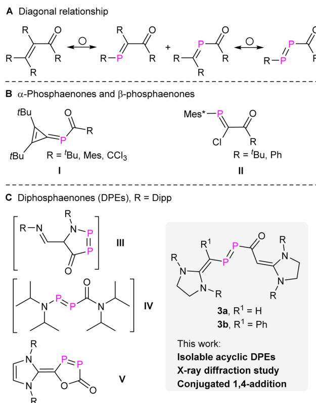
Fig. 1 (A) Diagonal relationship between enones and their phosphorus analogues. (B and C) Selected examples of \alpha -phosphaenones, \beta -phosphaenones, and diphosphaenones. Mes, 2,4,6-tri-methylphenyl; Mes*, 2,4,6-tri- tert -butylphenyl; Dipp, 2,6-di-isopropylphenyl.
