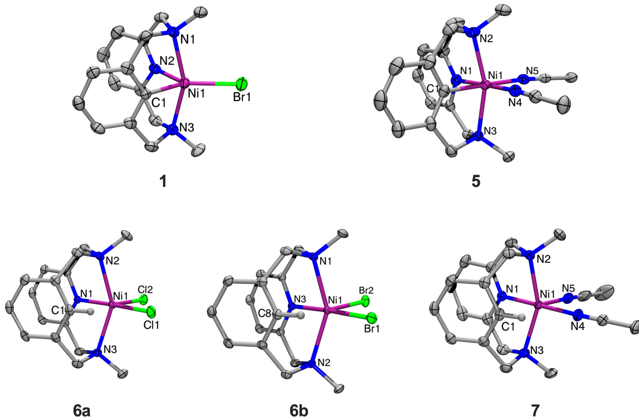
Fig. 1 ORTEPs (50% probability thermal ellipsoids) of complexes 1 , 5 , 6a , 6b , and 7 . For clarity, hydrogen atoms and counterions have been omitted. Selected bond distances (Å): 1 : Ni1–N1, 2.291(8); Ni1–N2, 1.981(7); Ni1–N3, 2.276(8); Ni1–C1, 1.954(9); Ni1–Br1, 2.372(2). 5 : Ni1–N1, 1.935(2); Ni1–N2, 2.152(2); Ni1–N3, 2.142(2); Ni1–N4, 1.983(2); Ni1–N5, 1.990(2); Ni1–C1, 1.921(2). 6a : Ni1–N1, 1.993(2); Ni1–N2, 2.233(2); Ni1–N3, 2.242(2); Ni1–C1, 2.539(2); Ni–Cl1, 2.312(5); Ni–Cl2, 2.329(6). 6b : Ni1–N1, 2.223(1); Ni1–N2, 2.255(1); Ni1–N3, 1.985(1); Ni1–C8, 2.482(2); Ni1–Br1, 2.455(4); Ni1–Br2, 2.478(4). 7 : Ni1–N1, 1.971(2); Ni1–N2, 2.179(2); Ni1–N3, 2.169(2); Ni1–N4, 2.023(2); Ni1–N5, 2.037(2); Ni1–C1, 2.412(2).
