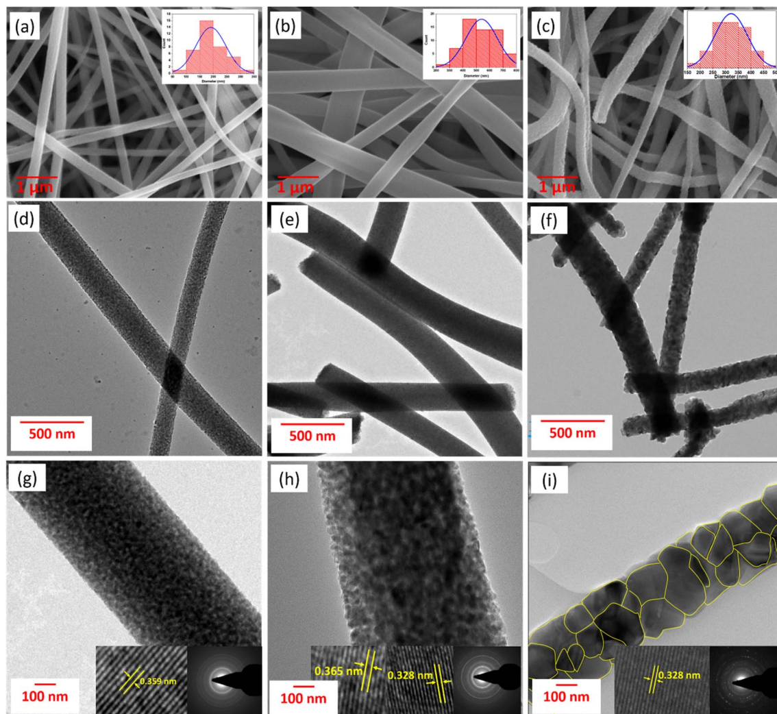
Fig. 2 SEM micrographs of (a) \text{TiO}_2 -A, (b) \text{TiO}_2 -AR and (c) \text{TiO}_2 -R. (d–f) TEM images and (g–i) HRTEM images (with SAED patterns as inset) of \text{TiO}_2 -A, \text{TiO}_2 -AR and \text{TiO}_2 -R, respectively.
