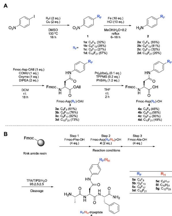
Scheme 1 (A) Synthesis of R_F -containing amino acids ( R_F -AAs) and (B) peptides ( R_F/R_H -tripeptides). Reaction conditions for the peptide synthesis: Fmoc-AAs-OH (4 eq.), COMU (4 eq.), oxyma (4 eq.), and DIPEA (8 eq.) for 1 h at r.t., then Fmoc group was deprotected by 20% piperidine/DMF for 5 min at r.t., OAll: allyl ester, DMSO: dimethyl sulfoxide, DCM: dichloromethane, MeOH: methanol, THF: tetrahydrofuran, DMF: dimethylformamide, TPPMS: sodium diphenylphosphino-benzene-3-sulfonate, TIPS: triisopropylsilane, TFA: trifluoroacetic acid, COMU: (1-cyano-2-ethoxy-2-oxoethylidenamino)dimethylamino-morpholino-carbenium hexafluorophosphate, oxyma: ethyl 2-cyano-2-(hydroxyimino)acetate, DIPEA: N,N -diisopropylethylamine.
