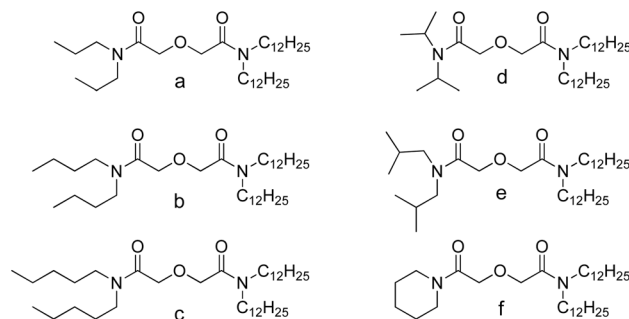
Fig. 3 Structures of the unsymmetrical diglycolamides investigated in this work: (a) PdDGA, (b) BdDGA, (c) PnDdGA, (d) iPDdGA, (e) iBdDGA, and (f) pipDdGA.
