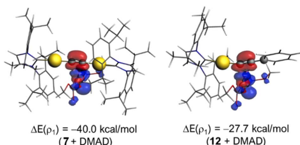
Fig. 12 Contour plots of the NOCV deformation densities \rho (isosurface value of 0.001 a.u.) and the associated energies \Delta E(\rho) (at a consistent C...C bond-forming distance of 2.1 Å) for the main orbital interaction occurring in the reaction of DMAD with 7 (left) and 12 (right). The electronic charge flows from red to blue. All data were computed at the ZORA-M06L-D3/DZP//SMD-M06L-D3/6-31G(d,p) &SDD(+f) level.
