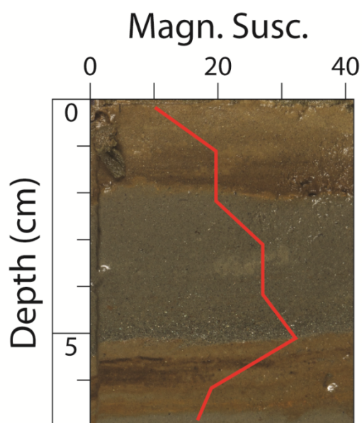
Figure 5: A turbiditic sediment layer (core A: 2-5 cm depth), clearly visible in the photo and indicated by higher magnetic susceptibility (red line), is overlaying the uppermost buried Fe/Mn layer (below 5 cm).
