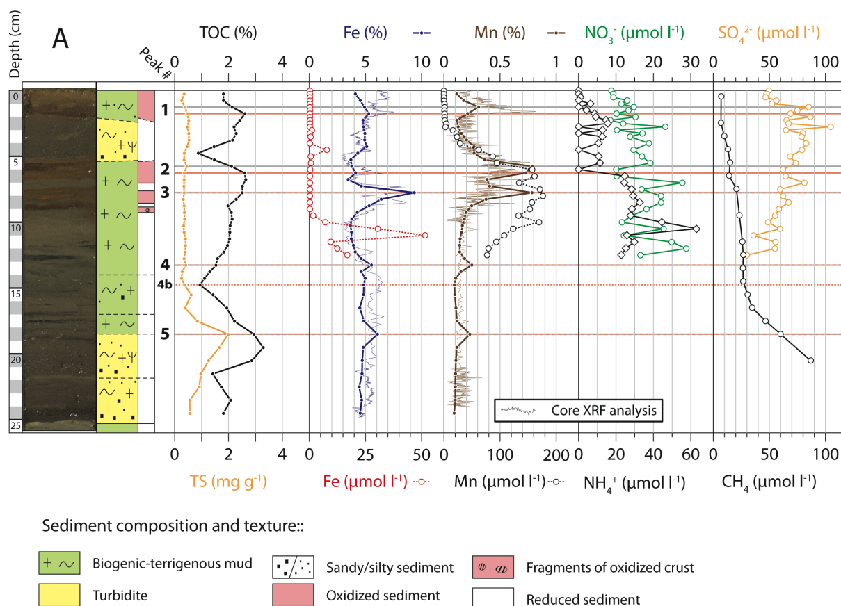
Figure 2: Core A, its lithology, composition, and the geochemical profiles as discussed in the present study. Fe and Mn oxide enrichments discussed in the text are numbered (#).
