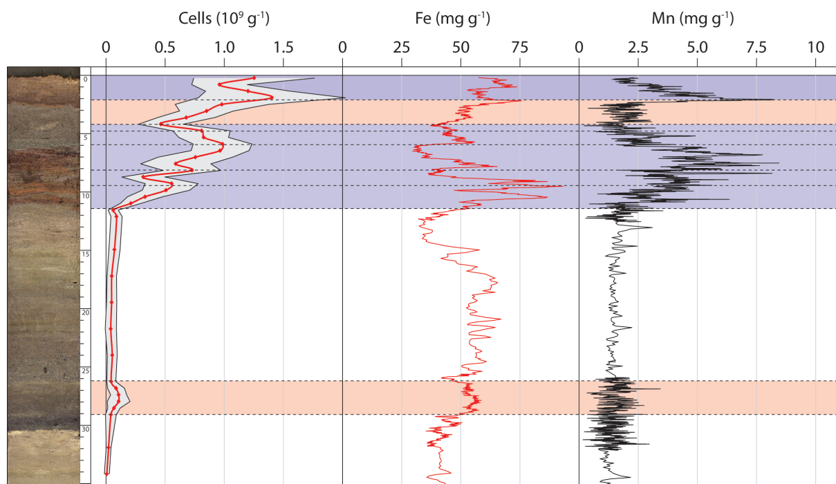
Figure 4: Depth profile of DAPI stained cells in the sediment (with standard deviation in grey). The core was taken close to the location of core A. Peaks at 2, 6, 9.5 and 28 cm depth confirm the heterogeneity of the sediment. The peaks coincides clearly with the visible Mn oxide (blackish) and Fe oxide (reddish) layers from the photograph as well as with the XRF scan reflecting Mn and Fe oxide levels. The top peak at 2 cm corresponds to the current oxic-anoxic interface.
