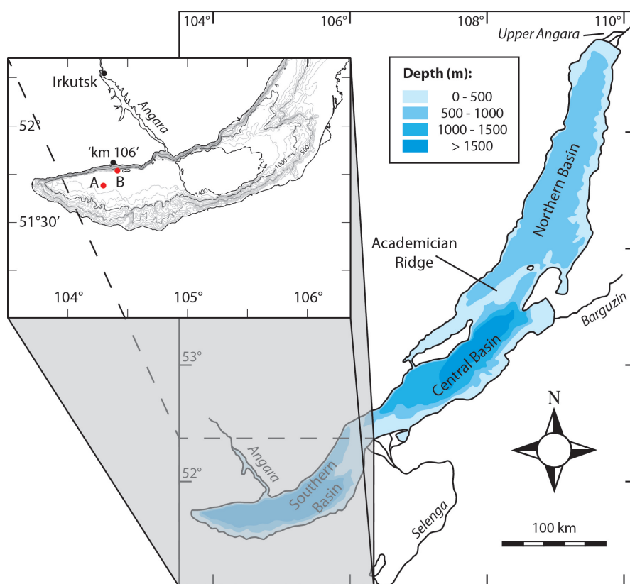
Figure 1: Map of Lake Baikal and a zoom into the Southern Basin relief. The coring sites A and B are indicated by red dots. Base camp (NEUTRINO station) was at the shore of the lake near the station 'km 106' of the Circum-Baikal Railway.
