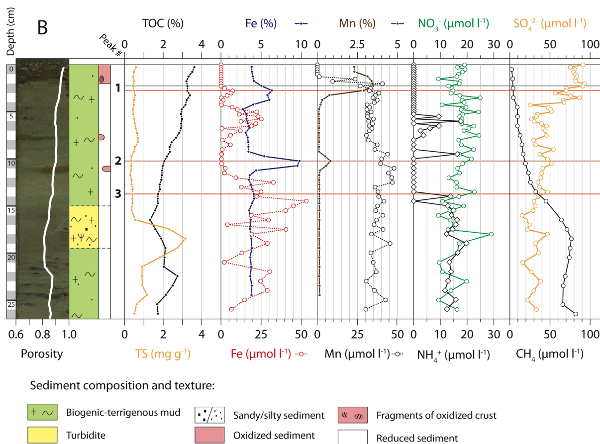
Figure 3: Core B, its lithology, composition, and the geochemical profiles as discussed in the present study. Fe and Mn oxide enrichments discussed in the text are numbered (#).
