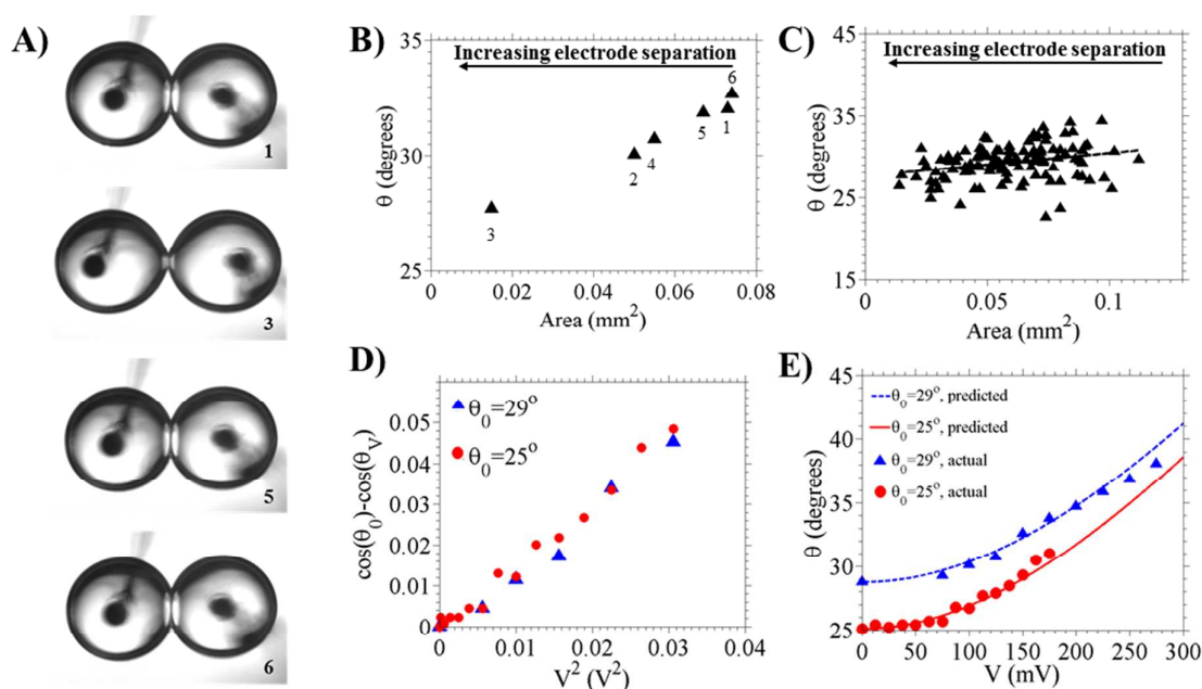
Figure 5. A) A DPhPC DIB at varying steps during Part 2 of an experiment where DIB area is mechanically varied by moving one electrode and changing the distance between droplets. B) \theta measured from images of the DIB at each area step. C) \theta measured from n > 100 images obtained at varying area steps with 13 separate DPhPC DIBs during C_M measurements. D) The change in the cosine of \theta as a function of voltage for a DPhPC DIB mechanically manipulated to obtain two different zero-volt contact angles: \theta_0 = 29^\circ and 25^\circ . E) Theoretical (“predicted”) and experimentally observed (“actual”) nominal \theta as a function of voltage for the trials shown in (D).
