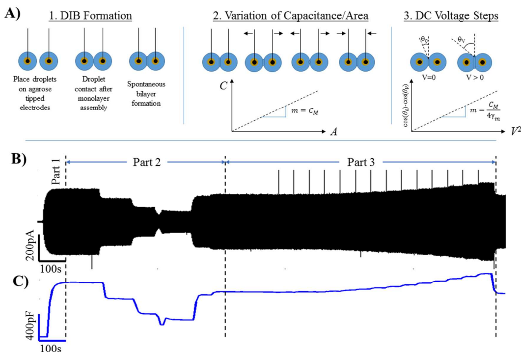
Figure 2. A) A three-part process is used to characterize DIBs: Part I represents bilayer formation; Part II represents the mechanical tuning of the bilayer area to determine specific capacitance; and Part III represents electrical tuning of the contact angle to determine monolayer tension via the Young-Lippmann equation (Equation 3). B) A typical current trace recorded during the course of an experiment in which all three parts are performed. C) Membrane capacitance versus time computed from the raw square current waveform shown in B).
