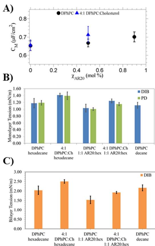
Figure 7. A) Values obtained from measurements of specific capacitance for bilayers as a function of the fraction of silicone oil added to the hexadecane oil phase. Error bars show \pm one standard deviation. Two lipid compositions are tested in the various oil mixtures: pure DPhPC, and DPhPC containing 20% (mol %) cholesterol. B) “DIB-YL” –monolayer tensions measured by monitoring Young-Lippmann related changes in DIB contact angle as voltage is increased. “PD” – monolayer tensions measured using the pendant drop method with a goniometer. C) Bilayer tensions for each lipid-oil combination, calculated using average observed contact angle (case specific) and the monolayer tension measured via the DIB-YL method.
