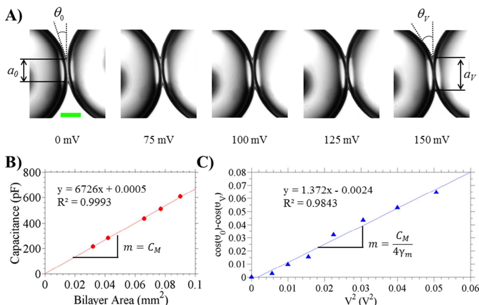
Figure 3. A) Representative images of a DPhPC DIB in decane during a Young-Lippmann test for monolayer and bilayer tensions (bottom-view images, scale bar represents 100 \mu\text{m} ). The DIB is allowed to equilibrate at each voltage before capturing any images used for contact angle measurements. The contact angle and the contact area increase with increasing voltage. This behavior is a result of reduction in bilayer surface tension by an amount equal to the energy stored on the capacitor. B) Results from specific capacitance measurement ( V=0 \text{ mV} , Part II in Fig. 2) C) The Young-Lippmann equation describes the linear relationship between applied bias voltage and the resulting change in the cosine of the contact angle. Experimental observation of contact angle at various applied voltages then allows for calculation of the monolayer tension. Parts B and C represent data obtained from a DPhPC DIB in hexadecane.
