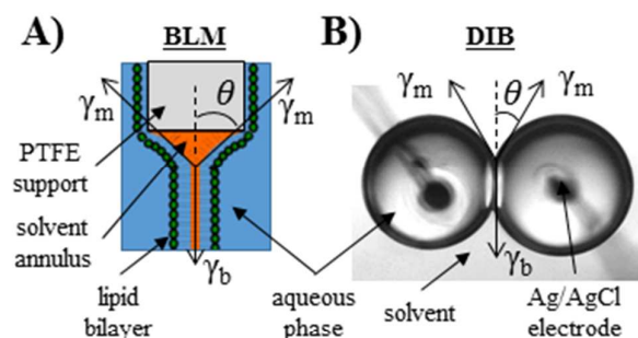
Figure 1. Common model membranes include the black lipid membrane (A) and the droplet interface bilayer (B). In both cases, the tension of the lipid bilayer that forms is in equilibrium with the vertical sum of the two opposing monolayer tensions.
