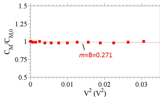
Figure 6. Normalized specific capacitance for a DPhPC DIB (hexadecane oil phase) as a function of applied voltage. C_{M,0} is the specific capacitance measured via dynamic capacitance/area changes with voltage clamped at 0mV (see Fig. 2, part II).
