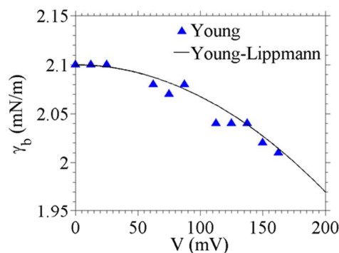
Figure 4. Bilayer tension ( \gamma_b ) as a function of applied voltage ( V ) for a DIB, calculated using the representative data presented in Fig. 3.
