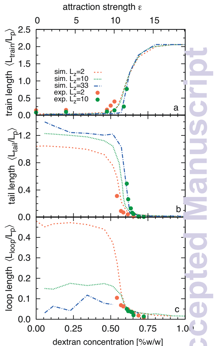
FIG. 2. The length of filament trains, tails and loops and their dependence on the attraction strength, \varepsilon (or equivalent depletant concentration C_p ), averaged over independent configurations and normalized by the filament persistence length L_p . a) Average train length \langle L_{\text{train}} \rangle / L_p . b) Average tail length \langle L_{\text{tail}} \rangle / L_p . c) Average loop length \langle L_{\text{loop}} \rangle / L_p . Filled circles correspond to experimental data and lines indicate simulation results. Chamber heights, L_z are specified in the figure legend. The simulation data are scaled onto depletant concentration, C_p , using \varepsilon = C_p/C were C = 16.75 .
