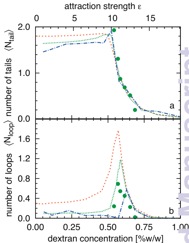
FIG. 4. a) Average number of tails \langle N_{tail} \rangle plotted as a function of the attraction strength, \varepsilon (or equivalent the depletion concentration C_p ). b) Average number of loops \langle N_{loop} \rangle as a function of \varepsilon . Symbols, lines and color coding is as in Fig. 2.
