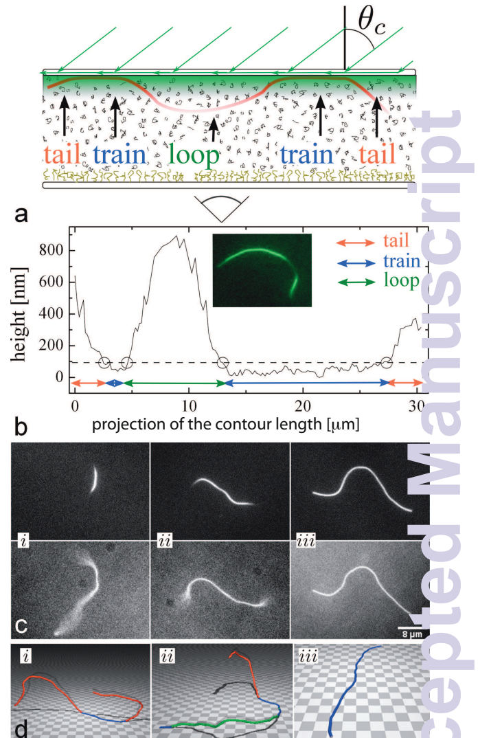
FIG. 1. TIRF microscopy determines 3D conformations of a fluctuating filament undergoing adsorption/desorption transition. a) Schematic of the experimental setup. An evanescent field is achieved by refracting laser through a prism above the critical angle \theta_c . The sample is viewed from below with a high numerical aperture (NA) objective. A polymer brush coating the coverslip surface ensures that filaments adsorb only on the top surface. b) The filament height plotted as a function of its position makes it possible to identify tails, trains and loops. The local height, h , is extracted from the filament intensity according to the relationship, h = -a \ln(I/I_0) where I is the intensity at a given height, I_0 the contour's maximum intensity (an offset is subtracted from both) and a is a decay constant of the evanescent field. Inset: Image of the filaments from which the height information is extracted. c) TIRF (top) and corresponding epi-fluorescence (bottom) images of adsorbed filaments at three different dextran concentrations corresponding to (i) the desorbed regime, (ii) the transition region and (iii) strongly adsorbed regime. For related movies see Ref. [36]. d) Snapshots of filament configurations obtained with computer simulations corresponding to three regime.
