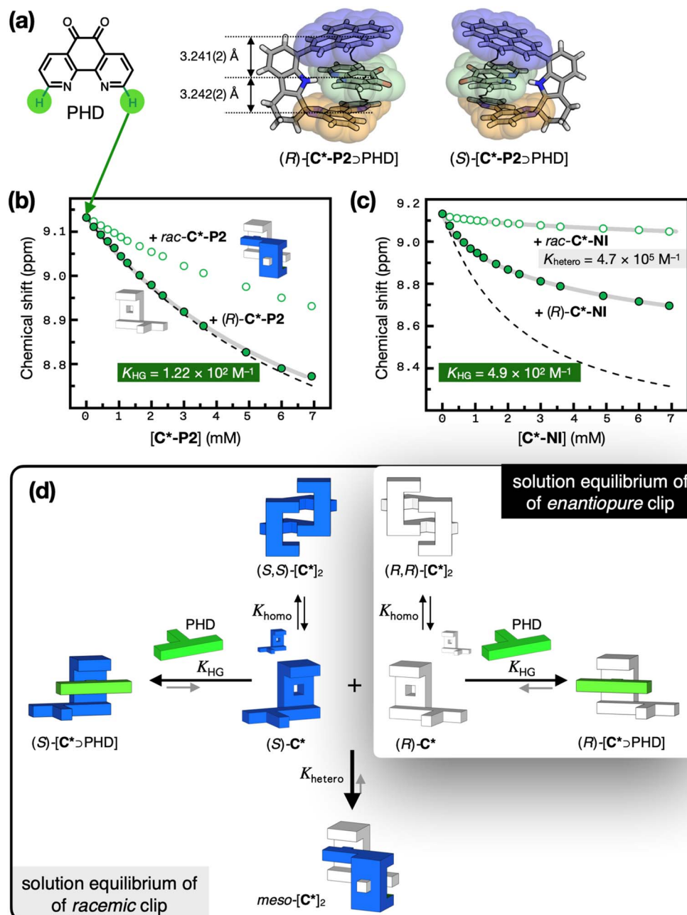
Fig. 6 (a) Chemical structure of PHD and capped-stick representation of the X-ray structure of (R)-[C*-P2 ⊃ PHD] and (S)-[C*-P2 ⊃ PHD] with vdW surfaces overlaid on the stacked aromatic regions, and ether chains simplified as wireframes. Changes in the chemical shifts of PHD proton resonances (denoted by green circles in the chemical structure; [PHD] 0 = 0.45 mM; T = 298 K) in CDCl 3 during titrations with (b) C*-P2, and (c) C*-NI. Experiments conducted with enantiopure clips are denoted by green filled circles, and those with racemic clips by green hollow circles. (d) Schematic representation of equilibrium between monomeric and dimeric hosts and host–guest complexes. The overlaid gray lines on (b) and (c) are theoretical fits that take into account homochiral dimerization ( K_{\text{homo}} ), host–guest complexation ( K_{\text{HG}} ), and, if applicable, heterochiral dimerization ( K_{\text{hetero}} ) of the hosts, as described in (d). Dashed lines in the plots (b) and (c) denote expected titration curves in the absence of host dimerization.
