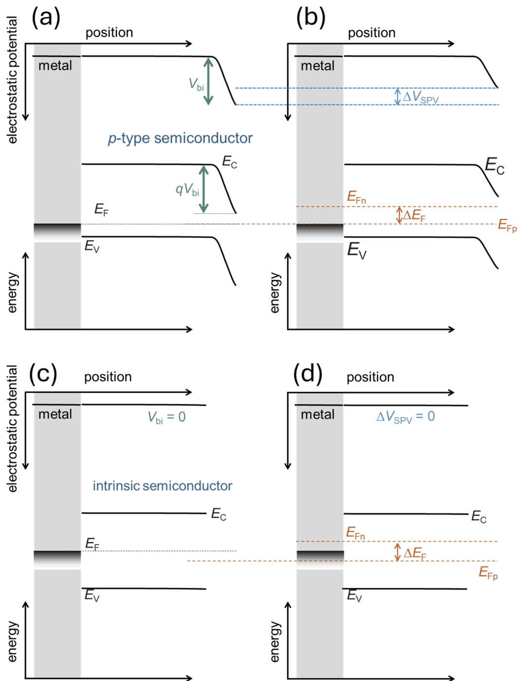
Fig. 20 Schematic to explain the difference between surface photovoltage \Delta V_{SPV} vs. Fermi level splitting \Delta E_F in doped (a and b) and undoped semiconductors (c and d). In the case of a p-type semiconductor forming an ohmic contact to a metal substrate, there is an electrostatic potential difference V_{bi} in equilibrium (a). Under non-equilibrium, low level injection conditions, the semiconductor will show a Fermi level splitting \Delta E_F and an electrostatic potential difference V_{bi} - V , where qV = \Delta E_F . Thus, a PL measurement to determine \Delta E_F , would provide the same information as the surface photovoltage. In case of an intrinsic semiconductor with blocking contacts (c) V_{bi} = 0 , and any illumination would still lead to zero electrostatic potential difference (d) as there is no symmetry breaking element in the system. Thus, in this case one could measure a PL but the SPV would be zero. Thus, the comparison of PL and SPV can be sensitive to the existence (or absence) of symmetry breaking elements that support charge separation.
