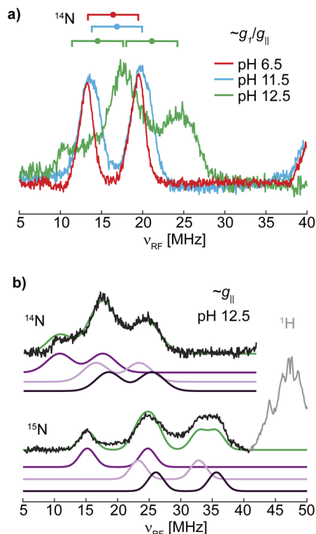
Fig. 6 (a) Overlay of the ^{14}\text{N} ENDOR spectra of LPMO-6.5, LPMO-11.5, and LPMO-12.5 collected along g_{\parallel}/g_{\perp} (10.900, 10.916, 11.096 G, respectively; also shown in Fig. 5 and S19†) with goalposts centered at A/2 and split by 2\nu_{\text{N}} . (b) Gaussian doublet fits of the ^{14}\text{N} and ^{15}\text{N} ENDOR with individual nitrogen doublet pairs and their sum (green) for ( ^{15}\text{N} )-LPMO-12.5.
