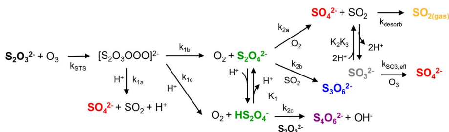
Scheme 1 Reaction mechanism for the oxidation of aqueous thiosulfate ( \text{S}_2\text{O}_3^{2-} ) by ozone ( \text{O}_3 ). Reprinted with permission from Deal, et al. 7 Copyright 2024 American Chemical Society.
