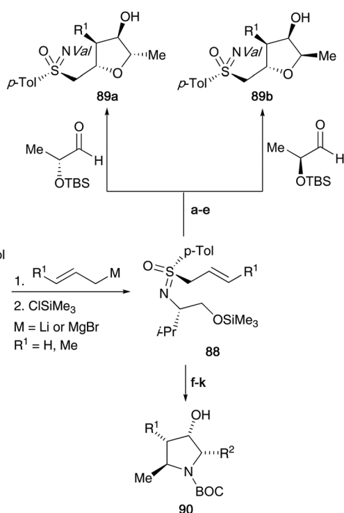
Scheme 23 Application of 2-alkenylsulfoximines 88 towards the construction of important organic heterocycles 89 and 90 . Reaction conditions: (a) n -BuLi, THF, -78 °C; (b) CPTi(O i Pr) 3 , 0 °C; (c) aldehyde, -78 °C; (d) (NH 4 ) 2 CO 3 ; (e) Bu 4 NF; (f) n -BuLi, toluene, -78 °C; (g) CPTi(O i Pr) 3 , 0 °C; (h) Fmoc-protected α-aminoaldehydes, -78 °C; (i) piperidine, 20 °C, (NH 4 ) 2 CO 3 , NH 4 Cl; (j) K 2 CO 3 , MeOH; BOC 2 O, NaHCO 3 ; (k) Sml 2 .
