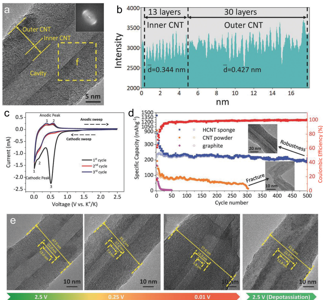
Fig. 20 (a) TEM image of a CNT. (b) Line profile obtained from the wall of a CNT. (c) CV curves of CNT sponge at 0.3 mV s -1 . (d) Cycling performance of CNT sponge, commercial CNT powder and graphite electrodes at a current density of 100 mA g -1 . (e) Ex situ TEM images of the CNT structure at different potassiation and de-potassiation potential in the first cycle. Reproduced from ref. 344 with permission from Wiley-VCH.
