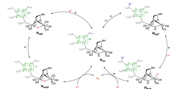
Fig. 20 Shortened catalytic cycle A from Fig. 3.11 and secondary cycle, which is based on bridging hydrides. Red protons: catalytic PTP, blue proton: accessory PTP. * \text{H}_{\text{ox}}\text{H} might be involved in this conversion.
