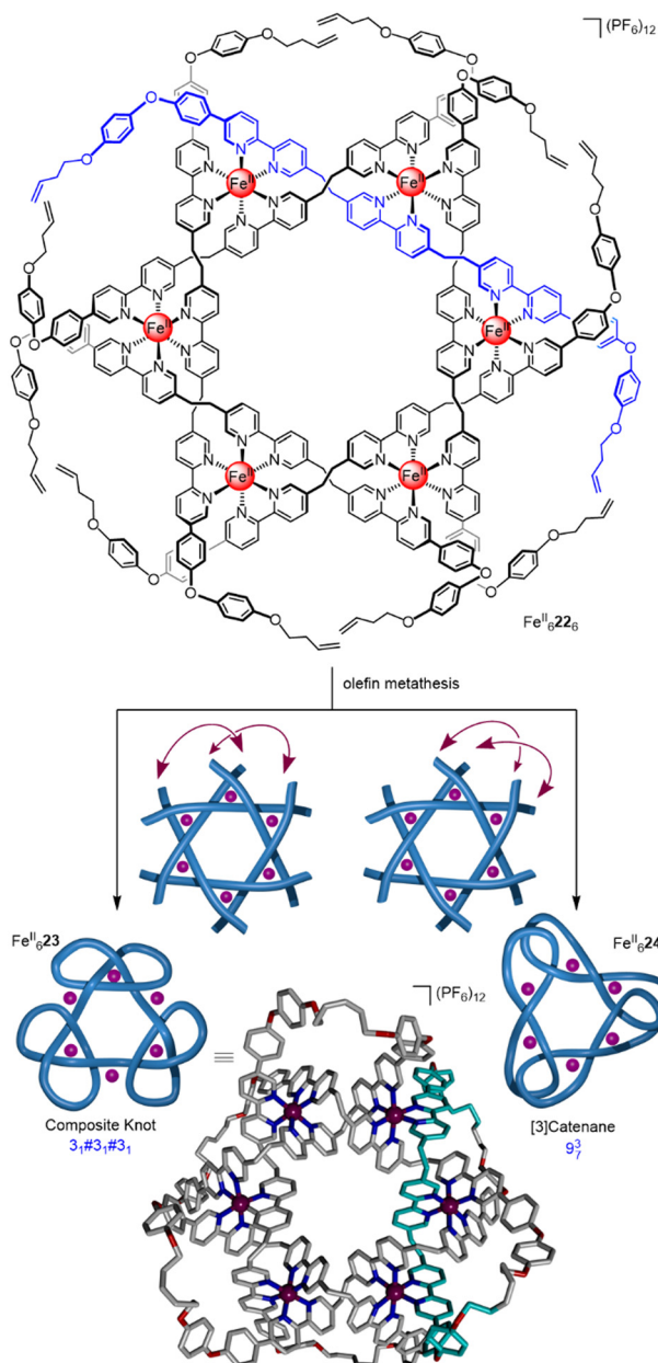
Fig. 8 A hexameric circular helicate and its closure to give molecular composite knot Fe 6 II 23 and link Fe 6 II 24. 58
