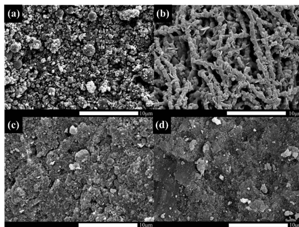
Fig. 1 SEM image of CoNPs (a), CoNWs (b), CoNPs@CoAl-LDHs/Fe 3 O 4 (c) and CoNWs@CoAl-LDHs/Fe 3 O 4 (d).
