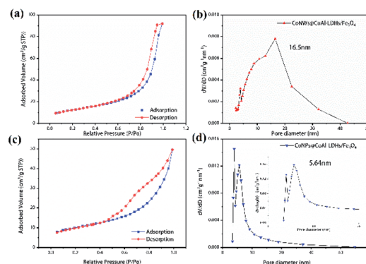
Fig. 4 N 2 adsorption-desorption isotherms and the BJH pore size distribution of CoNWs@CoAl-LDHs/Fe 3 O 4 (a and b) and CoNPs@CoAl-LDHs/Fe 3 O 4 (c and d).
