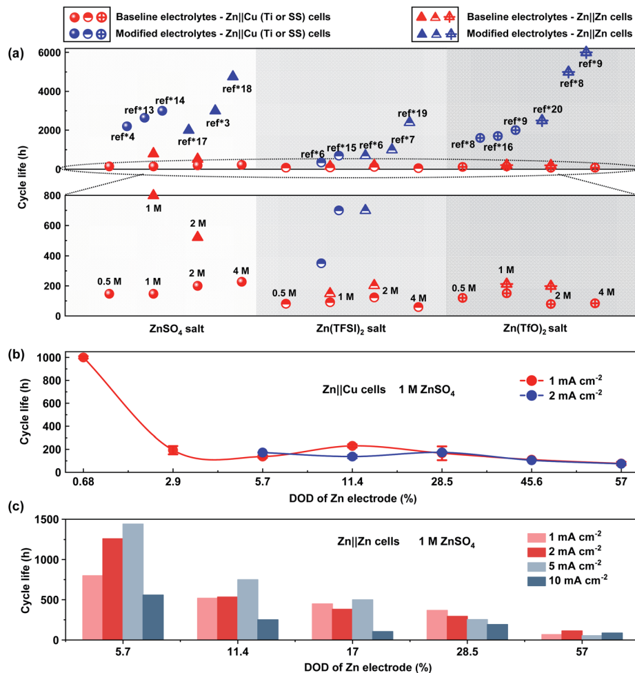
Fig. 2 Cycle life curves of Zn anodes in \text{Zn||Cu} (Ti or SS) half cells and \text{Zn||Zn} symmetric cells under different test conditions. (a) Comparison between the baseline \text{ZnSO}_4 , \text{Zn(TFSI)}_2 , and \text{Zn(TfO)}_2 based aqueous electrolytes with different salt concentrations (red circles: \text{Zn||Cu} cells; red triangles: \text{Zn||Zn} cells; 1 mA \text{cm}^{-2} and 1 mA h \text{cm}^{-2} ) and modified aqueous electrolytes in published reports under different test conditions (blue circles: \text{Zn||Cu} cells; blue triangles: \text{Zn||Zn} cells; the "ref*" represents the references in the ESI,† and the detailed test conditions of these references are described in Tables S2 and S3†); (b) different DODs of Zn anodes with a 1 M \text{ZnSO}_4 electrolyte at 1 mA \text{cm}^{-2} and 2 mA \text{cm}^{-2} in \text{Zn||Cu} half cells; (c) different DODs of Zn anodes with a 1 M \text{ZnSO}_4 electrolyte at different current densities in \text{Zn||Zn} cells. Note that the cycle life of baseline electrolytes in Fig. 2a and the experimental data in Fig. 2b and c are re-evaluated with 30 \mu\text{m} and 250 \mu\text{m} Zn electrodes, and the detailed experimental results are listed in Table S4–S6.†
