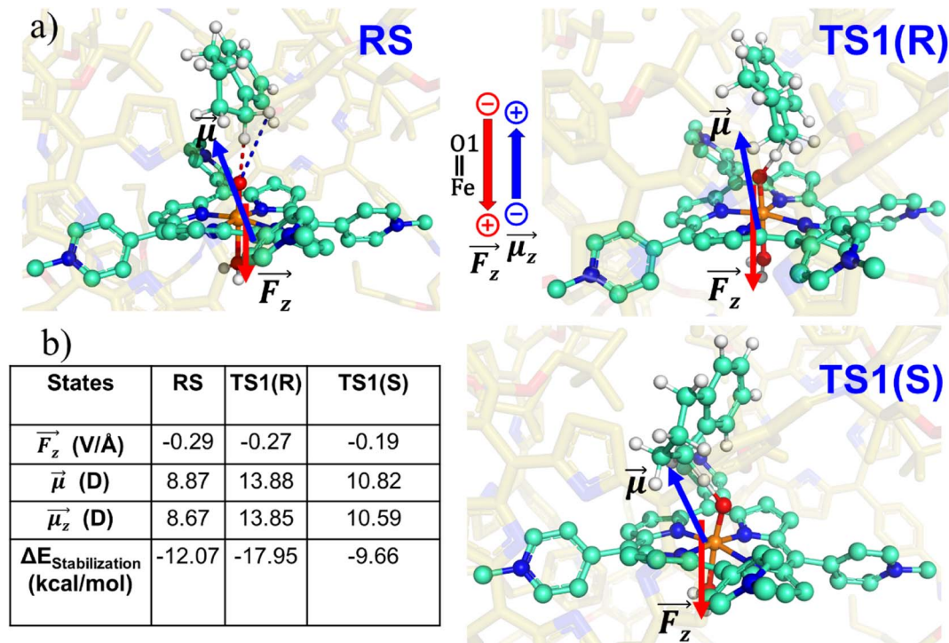
Fig. 8 (a) RS, TS1-R and TS1-S states showing the direction of local electric field (LEF) and dipole moment. (b) Calculated \text{LEF}_z , dipole moments, and stabilization energies. Note that we have a GAUSSIAN convention to define the direction of electric fields and dipole moments. Dipole moments have been calculated for \text{H}_2\text{O}-\text{Fe}=\text{O} , porphyrin and TLN.
