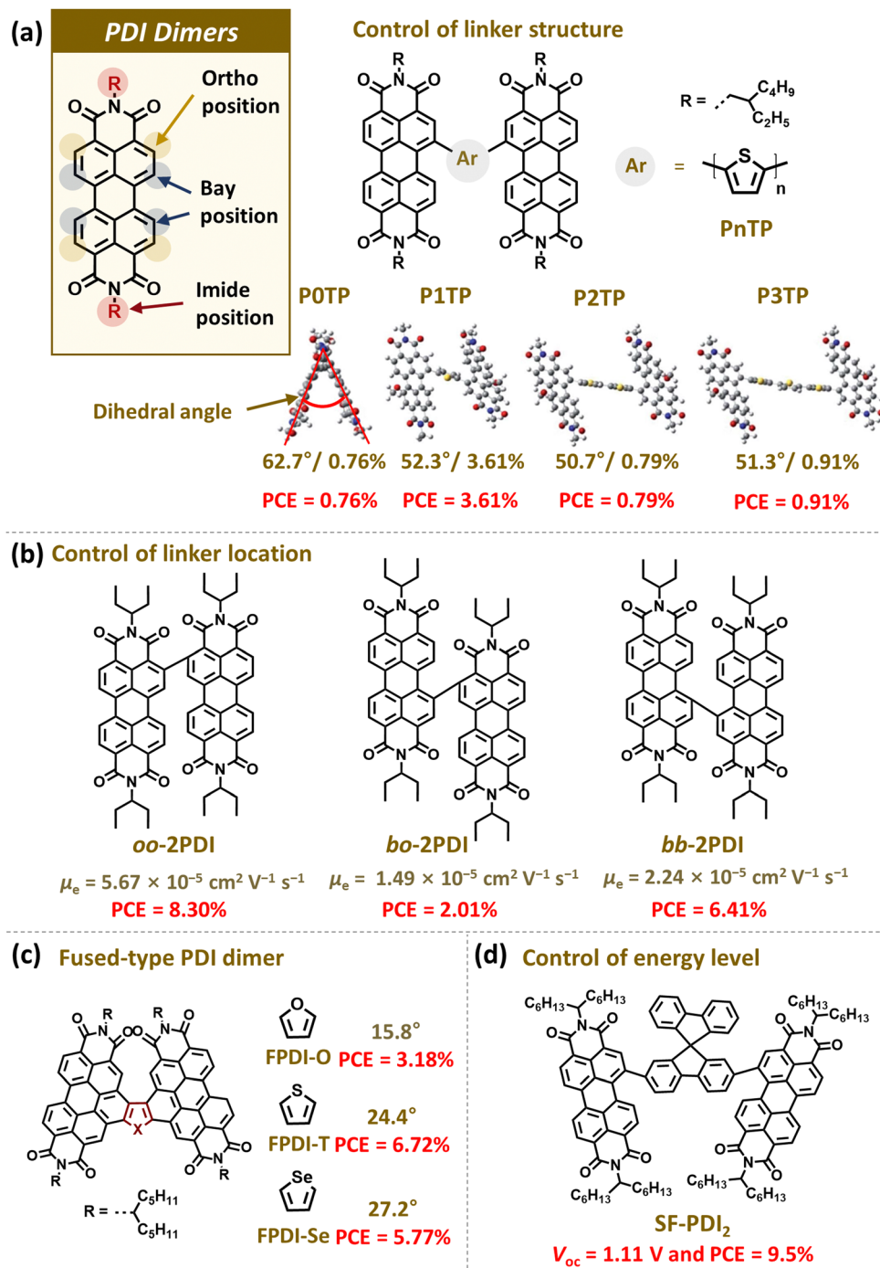
Fig. 5 Representative examples of PDI-based dimer acceptors; (a) POTP, P1TP, P2TP, and P3TP, (b) oo -2PDI, bo -2PDI, and bb -2PDI, (c) FPDI-O, FPDI-T, and FPDI-Se, and (d) SF-PDI 2 . Reproduced from ref. 121 with permission from the Royal Society of Chemistry, copyright 2024.
