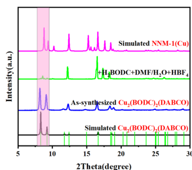
Fig. 3 The variation of PXRD patterns during the post-synthesis of NNM-1(Cu) with Cu_2(BODC)_2(DABCO) as the raw material.
