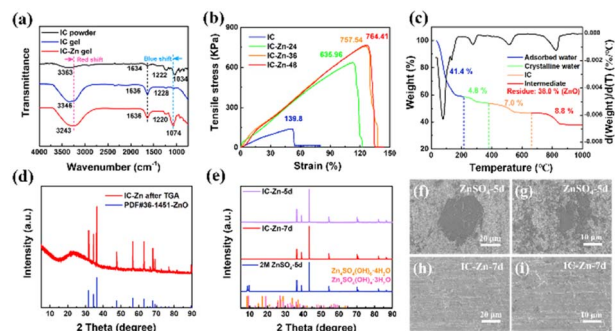
Fig. 2 (a) FT-IR spectra of IC-Zn gel, IC gel and IC powder. (b) Tensile curves of IC-Zn- T gel electrolytes with changing ion exchange time (IC-Zn- T , T = 0 h, 24 h, 36 h, 48 h). (c) TGA curve of IC-Zn gel electrolyte. (d) XRD pattern of IC-Zn after TGA. (e) XRD patterns of Zn foils for corrosion test. SEM images of (f and g) \text{ZnSO}_4 \cdot 5\text{d} and (h and i) IC-Zn-7 d (Zn foil soaked in IC-Zn for 7 days).
