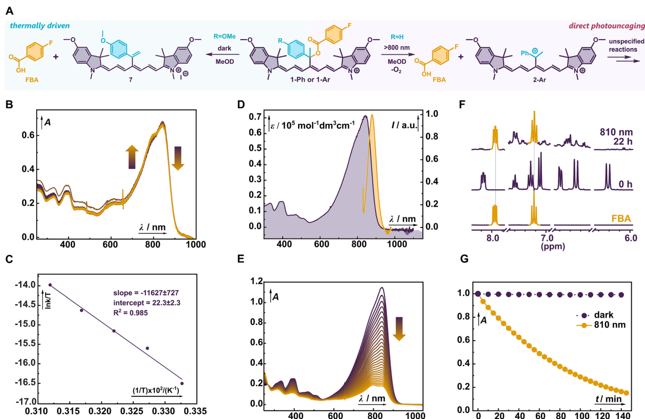
Fig. 2 (A) Photouncaging of FBA from 1-Ph under \text{O}_2 -free conditions (left) and thermally-driven elimination of FBA from 1-Ar (right). (B) Thermal decomposition of 1-Ar in MeOH at rt over 2 hours period by UV-vis spectroscopy (violet to yellow). (C) Eyring analysis of the thermally-driven elimination from 1-Ar . (D) UV-vis (violet) and emission (yellow) spectra of 1-Ph in MeOH. (E) NIR (820 nm) irradiation of 1-Ph in MeOH at ambient conditions, followed by UV-vis spectroscopy (violet to yellow). (F) ^1\text{H} NMR spectra of 1-Ph irradiated in \text{CD}_3\text{OD} at 810 nm under \text{O}_2 -free conditions. (G) Kinetic traces of 1-Ar irradiated at 820 nm (yellow) and in the dark (violet).
