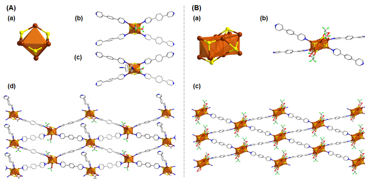
Fig. 2 (A) Structural architecture of \text{Cu}_6 -d pb (a) \text{Cu}_6 cluster node geometry and the attachment of four thiolate groups, (b) and (c) attachment of linker molecules and \text{CF}_3\text{COO}^- units, (d) 2D architecture of the \text{Cu}_6 -d pb CAM. (B) Structural architecture of \text{Cu}_{10} -d pb (a) \text{Cu}_{10} cluster node geometry and the attachment of four thiolate groups, (b) attachment of linker molecules and \text{CF}_3\text{COO}^- units, (c) 2D architecture of the \text{Cu}_{10} -d pb CAM. Hydrogen atoms and the associated solvent molecules are removed for the clarity. Color legend: Cu, brown; S, yellow; O, red; F, green; N, blue; C, grey stick.
