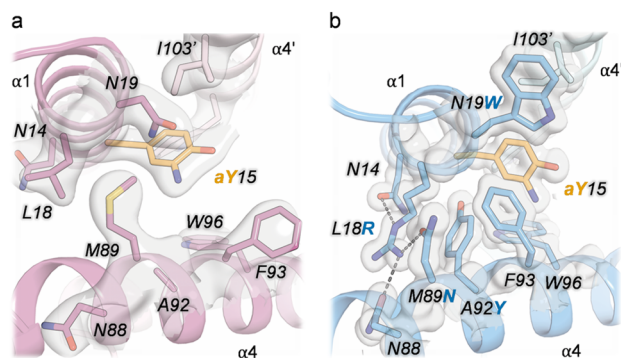
Fig. 3 Close-up views of the crystal structures of LmrR_V15aY (a) and LmrR_V15aY_RNYW_KK (b), highlighting 2Fo-Fc electron densities for selected residues (contoured at 1σ). Hydrogen bonds are displayed as dotted black lines. The mutations L18R, M89N, A92Y and N19W in the evolved variant result in an increased close packing of side chains of helices α1 and α4, achieved via the formation of hydrophobic contacts, aromatic stacking interactions and hydrogens bonds.
