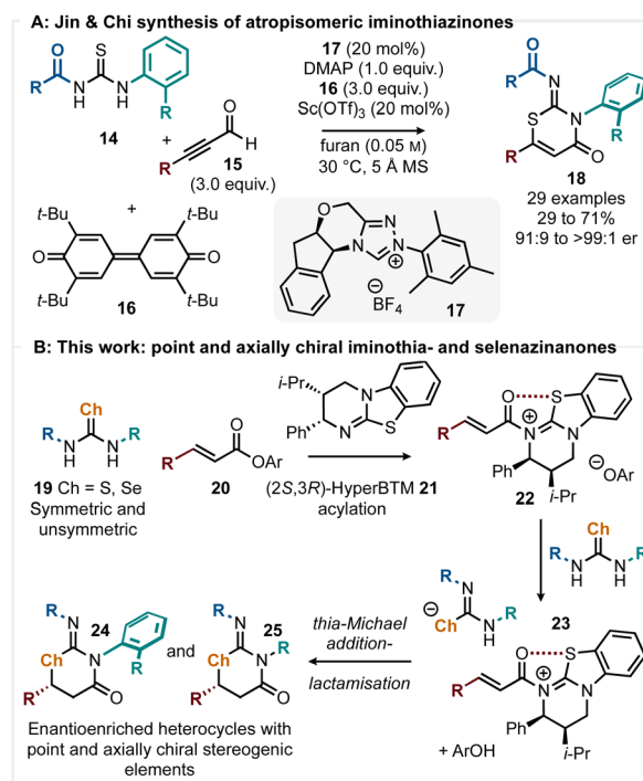
Scheme 2 (A) NHC-catalysed synthesis of atropisomeric iminothiazinones. (B) This work: isothioureia catalysed preparation of point and axially chiral heterocycles.
