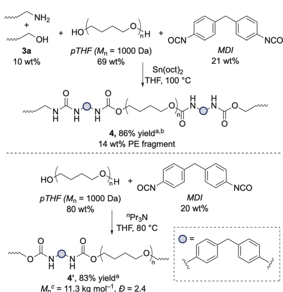
Scheme 2 Synthesis of PUUs through polymerization of alcohol- and amine-terminated LDPE fragments with MDI and p THF. a Yield with respect to mass. b We were unable to characterize the resulting material by gel-permeation chromatography (GPC) because of its insolubility in THF at 35 °C, DMF at 55 °C, or 1,2,4-trichlorobenzene at 135 °C. c Absolute molecular weight was calculated following detector calibration with a single narrow poly(styrene) standard.
