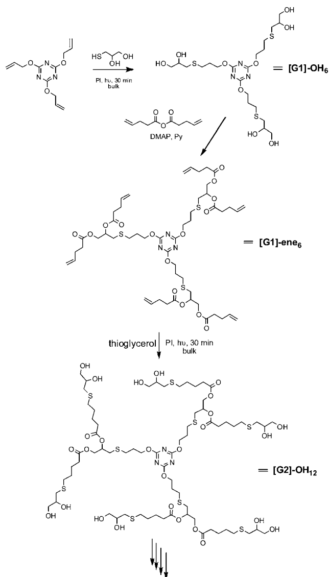
Scheme 10 Photochemical and thermal radical thiol-ene modification of pendent side-chains in styrenic, methacrylic and polyester-based copolymers.
