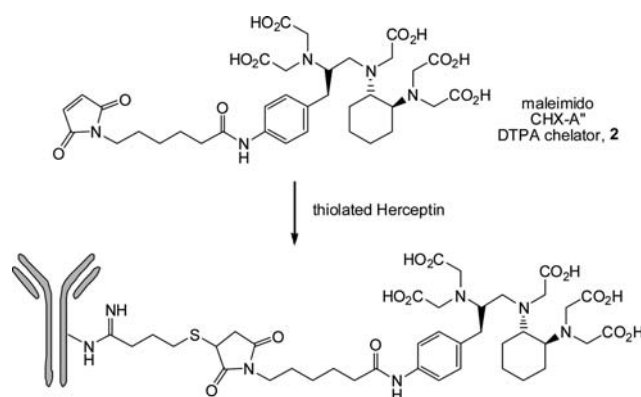
Scheme 31 Conjugation of a maleimide-functional chelator to the monoclonal antibody Herceptin as a facile route to bioconjugates for radioimmunoassay and radioimmunotherapy applications.
