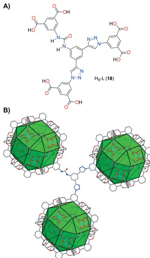
Fig. 6 A) Structure of the hexacarboxylic acid H 6 -L (18) . B) Single crystal structure of the (3,24)-connected rht -topological framework in Cu-UBTA. Tetragonal space group I4/m , unit cell dimensions a = b = 31.4206 Å, c = 44.8239 Å. BET surface area = 3134 m 2 g −1 . Adapted with permission from ref. 55. Copyright © Royal Society of Chemistry.
