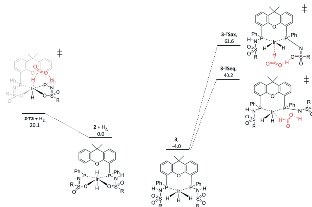
Fig. 4 DFT-calculated potential energy diagram of hydride transfer to \text{CO}_2 from complexes 2 and 3 . \Delta G_{298\text{K}}^0 in \text{kcal mol}^{-1} , \text{R} = \text{phenyl} (Turbomole, 17 BP86, def2-TZVP).
