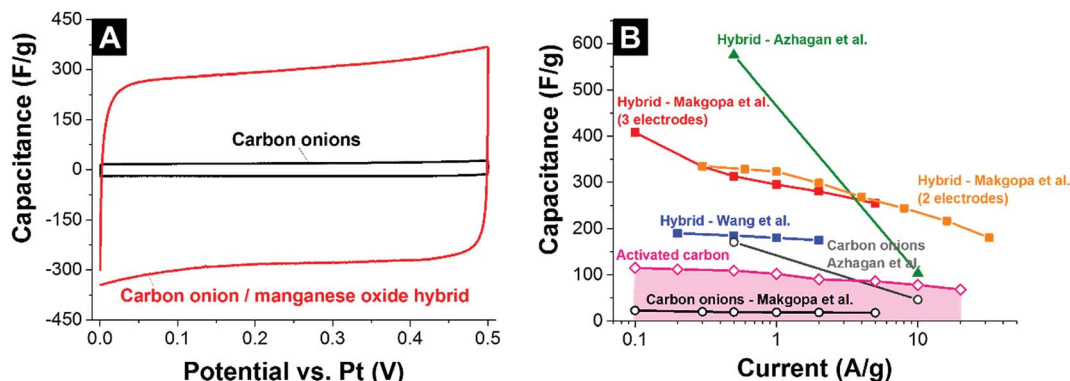
Fig. 13 (A) Cyclic voltammogram of carbon onions and carbon onion/manganese oxide nano hybrids in 1 M \text{Na}_2\text{SO}_4 . 135 (B) Rate handling plot of different types of carbon onions and carbon onion/manganese oxide composites. Makgopa et al. : nanodiamond-derived carbon onions coated in a hydrothermal reaction with manganese oxide; 1 M \text{Na}_2\text{SO}_4 electrolyte. 135 Azhagan et al. : burning ghee-derived carbon onions coated using a microwave assisted hydrothermal reaction; 0.5 M \text{H}_2\text{SO}_4 electrolyte. 86 Borgohain et al. : nanodiamond-derived carbon onions were combined with polydiallyldimethylammonium chloride (PDPA), and delaminated-manganese oxide by a sequential chemical deposition technique; 1 M \text{Na}_2\text{SO}_4 electrolyte. 136 Wang et al. : phenolic resin-derived carbon onions were hydrothermally coated with manganese oxide; 1 M \text{Na}_2\text{SO}_4 electrolyte. 137 Activated carbon electrodes were prepared using 5% PTFE as a binder and measured in 1 M \text{Na}_2\text{SO}_4 using a full cell set up.
