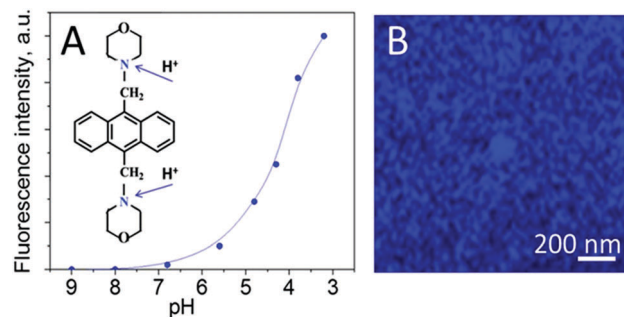
Fig. 3 (A) Calibration of fluorescent pH indicator, 4,4'-(anthracene-9,10-diyl)dimethanediyl)dimorpholine, that exhibits a \text{pK}_a \sim 5.1 , and initial chemical formula showing the protonation sites; (B) confocal fluorescent images of the \text{TiO}_2 surface immediately after irradiation.
