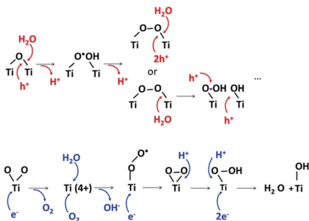
Fig. 2 Possible reorientation of titania groups and water under irradiation and reactions with photogenerated photohole ( \text{h}^+ ) and photoelectron ( \text{e}^- ).
