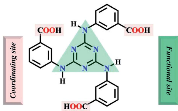
Scheme 1 The semi-rigid organic ligand H_3TATMA .
