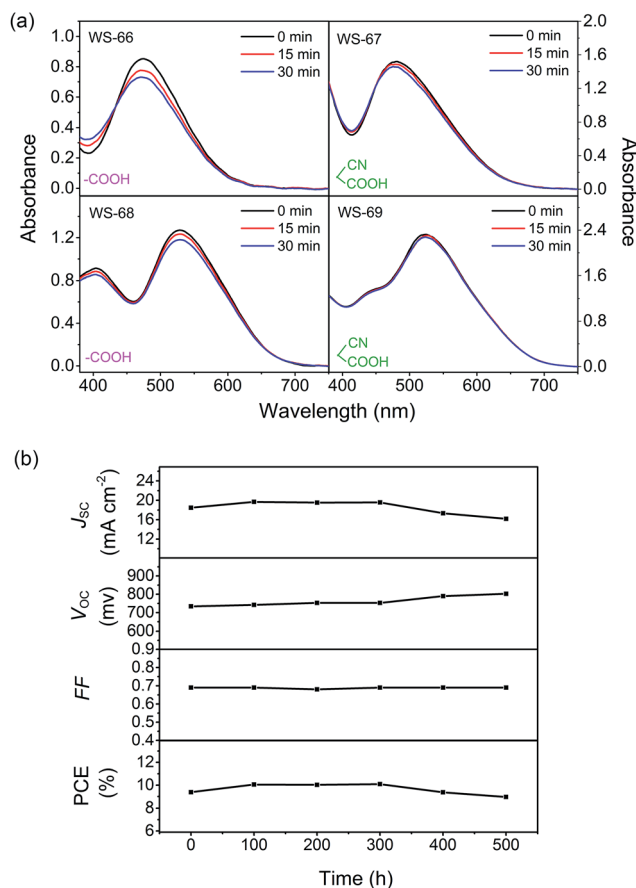
Fig. 9 Dyes WS-66, WS-67, WS-68 and WS-69 adsorbed on \text{TiO}_2 films before and after light irradiation for 15 and 30 min (a), evolution of photovoltaic performance parameters for DSSCs based on cosensitization of WS-69 with WS-5 under visible-light soaking (b).
