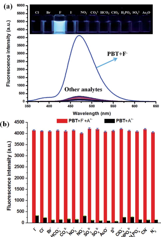
Fig. 6 (a) Fluorescence spectra of PBT in the presence of various anions. [PBT] = 10\ \mu\text{M} , [A_n^-] = 20\ \mu\text{M} , in a mixture of THF and Tris buffer solution (pH 8.0), (1 : 9, v/v), \lambda_{\text{ex}} = 335\ \text{nm} , \lambda_{\text{em}} = 470\ \text{nm} . Inset: direct observation of fluorescence emission difference of the probe PBT ( 10\ \mu\text{M} ) under UV irradiation (365 nm) in the presence of different anions. Left to right: \text{Cl}^- , \text{Br}^- , \text{I}^- , \text{F}^- , \text{NO}_2^- , \text{CO}_3^{2-} , \text{HCO}_3^- , \text{ClO}_4^- , \text{H}_2\text{PO}_4^- , \text{SO}_4^{2-} and \text{AcO}^- . (b) The selectivity of PBT in the presence of various anions.
