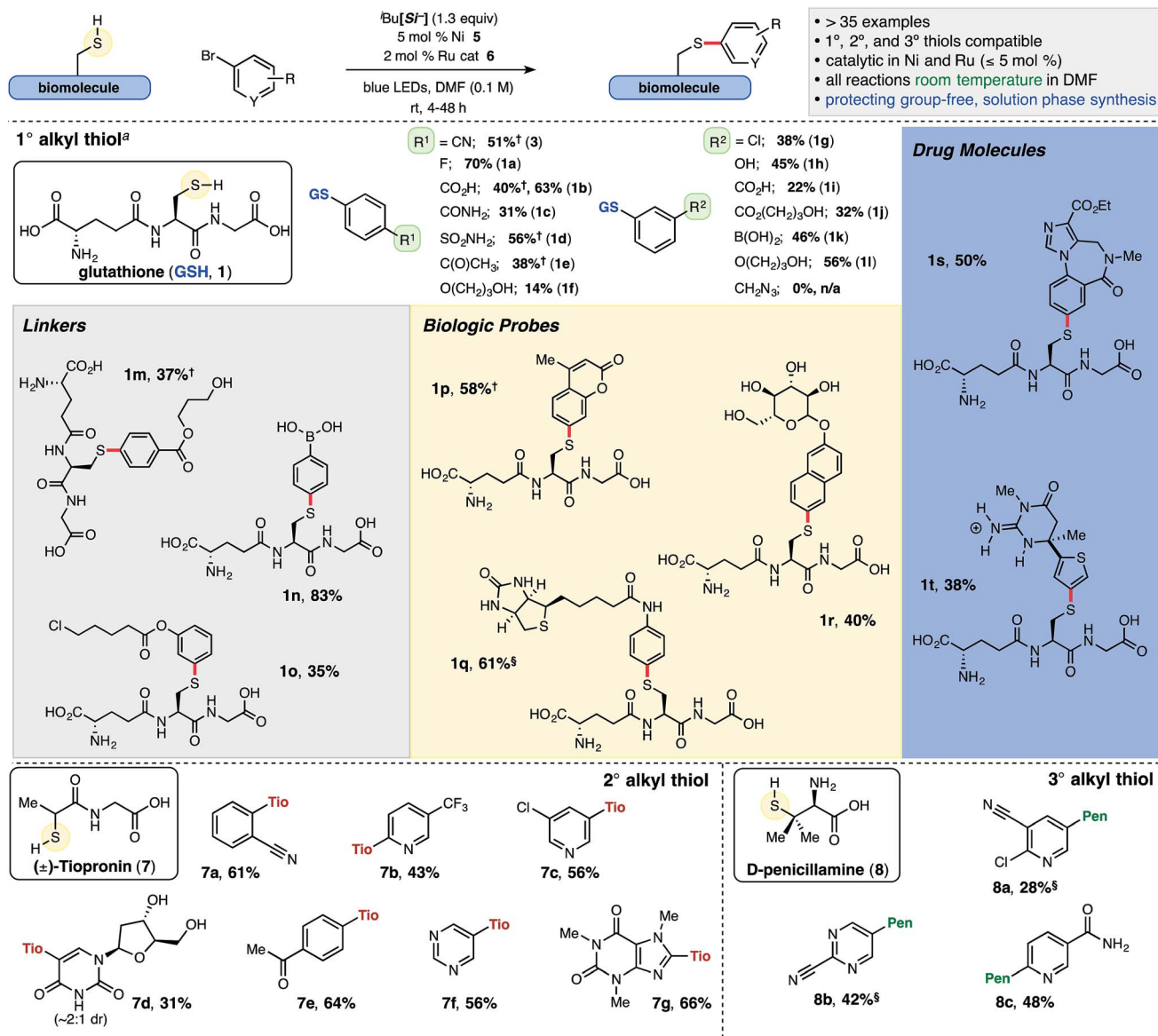
Chart 1 Ni/Photoredox thioarylation reaction and scope of various thiol and arene small molecules. \text{Bu[Si}^-\text{]}^- = diisopropylammonium bis(catechol)isobutylsilicate. DMF = N,N -dimethylformamide. Reactions conducted with 0.1 mmol thiol and ArBr, unless otherwise noted; isolated yields are reported (TFA salt omitted for clarity, see ESI† for additional details). a 0.12 mmol GSH employed. § 2 equiv. ArBr was employed. † The adduct was filtered following precipitation from the aqueous solution.
