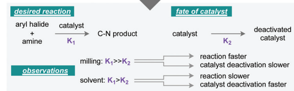
Scheme 3 (A) Synthesis of Vortioxetine featuring the mechanochemical Buchwald–Hartwig reaction. (B) reduced catalyst loading for the mechanochemical Buchwald–Hartwig amination. (C) robustness of these conditions under solvent based and solvent-free conditions. a Yield was determined by GC using mesitylene as internal standard. b Isolated yield.
