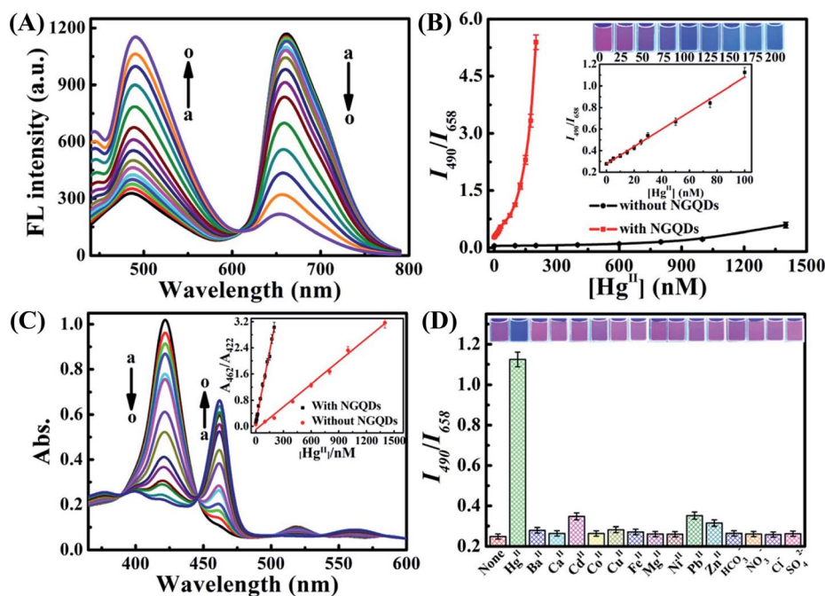
Fig. 37 (A) Fluorescence spectra of 5.0 \mu\text{M} 5,10,15,20-tetrakis(1-methyl-4-pyridinio)porphyrin tetra( p -toluenesulfonate) (TPyP) after the addition of 20 \mu\text{g L}^{-1} N-GQDs, 40 \mu\text{M} \text{Mn}^{II} , and different concentrations of \text{Hg}^{II} ranging from 0 to 200 nM. (B) Plot of the fluorescence ratio ( I_{490}/I_{658} ) vs. \text{Hg}^{II} concentrations (0–200 nM) in the presence or absence ( \text{Hg}^{II} concentrations of 0 to 1400 nM) of N-GQDs. Inset shows photographs corresponding to the \text{Hg}^{II} concentrations and the plot of ( I_{490}/I_{658} ) vs. \text{Hg}^{II} concentration (0–100 nM) in the presence of N-GQDs. (C) Absorption spectra of 5.0 \mu\text{M} TPyP after the addition of 40 \mu\text{M} \text{Mn}^{II} , 20 \mu\text{g L}^{-1} N-GQDs, and different concentrations of \text{Hg}^{II} ; inset shows plots of A_{462}/A_{422} vs. \text{Hg}^{II} concentration with and without N-GQDs. (D) The selectivity for \text{Hg}^{II} among different interfering analytes. The fluorescence quenching efficiency ( I_{490}/I_{658} ) of 5.0 \mu\text{M} TPyP after the addition of 40 \mu\text{M} \text{Mn}^{II} , 100 nM \text{Hg}^{II} and 20 \mu\text{g L}^{-1} N-GQDs and other interfering ions, including \text{Ba}^{II} , \text{Cd}^{II} , \text{Co}^{II} , \text{Cu}^{II} , \text{Fe}^{II} , \text{Ni}^{II} , \text{Pb}^{II} , \text{Zn}^{II} , \text{HCO}_3^- , \text{Cl}^- at 500 nM concentration; \text{Mg}^{II} , \text{SO}_4^{2-} , \text{NO}_3^- at 100 \mu\text{M} concentration; and \text{Ca}^{II} at 200 \mu\text{M} concentration; inset shows photographs of the fluorescence changes under 365 nm UV light. [Reprinted with permission from ref. 705, D. Peng, L. Zhang, R.-P. Liang and J.-D. Qiu, Rapid Detection of Mercury Ions Based on Nitrogen-Doped Graphene Quantum Dots Accelerating Formation of Manganese Porphyrin, ACS Sens. , 2018, 3, 1040–1047. Copyright© American Chemical Society.]
