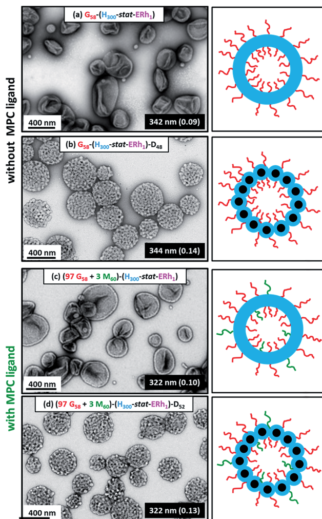
Fig. 3 Representative TEM images (and corresponding hydrodynamic diameters and DLS polydispersities) obtained for fluorescently-labeled (a) smooth G_{58}-(H_{300}\text{-stat-ERh}_1) diblock copolymer vesicles, (b) framboidal G_{58}-(H_{300}\text{-stat-ERh}_1)\text{-D}_{48} triblock copolymer vesicles, (c) smooth (97 G_{58} + 3 M_{60})-(H_{300}\text{-stat-ERh}_1) diblock copolymer vesicles and (d) framboidal (97 G_{58} + 3 M_{60})-(H_{300}\text{-stat-ERh}_1)\text{-D}_{52} triblock copolymer vesicles synthesized at pH 7.4 under sterile conditions. Corresponding color-coded schematic cartoons are also shown for each type of vesicle.
