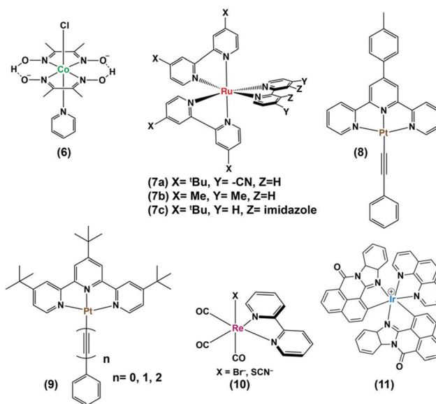
Fig. 2 Structures of various noble metal-based photosensitizers (7–11) used with cobaloxime derivatives, such as (6) for photocatalytic hydrogen evolution in homogeneous condition.
