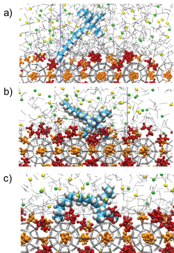
Fig. 17 Snapshots of molecular-dynamics simulation of AA molecule adsorption phenomenon onto the gas hydrate surface for three different kinds of molecular interactions with surface active species at the interface: (a) solely the long hydrocarbon tail of the AA molecule interacts with the hydrate surface, (b) solely the ionic head of the AA molecule has binding affinity to the hydrate surface, and (c) the AA molecule interacts with hydrate surface through simultaneously head and tail bindings to the surface (adapted with permission from Mehrabian et al. 1103 Copyright 2018 American Chemical Society).
