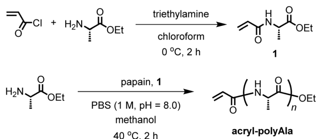
Scheme 1 Synthesis of an acrylamide terminal-modifying agent ( 1 ) and terminal-functionalized poly(L-alanine) via papain-catalyzed chemoenzymatic polymerization in the presence of 1 as a terminal modifier.
