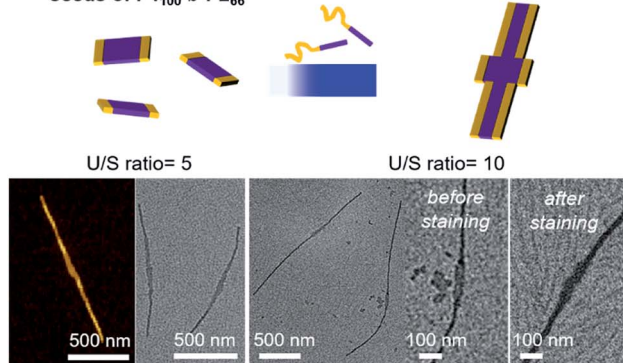
Fig. 7 More complex BCMs were prepared by (a) adding a unimer P3 25 -b-P2 22 having a different block to P1 50 -b-P2 22 seed (BCM1) and (b) adding a unimer ( P1 50 -b-P2 22 ) to a wider seed ( P1 100 -b-P2 66 ) to produce BCM2 with different widths. The number in an image (a) indicates "the average L_n and its length dispersity".
