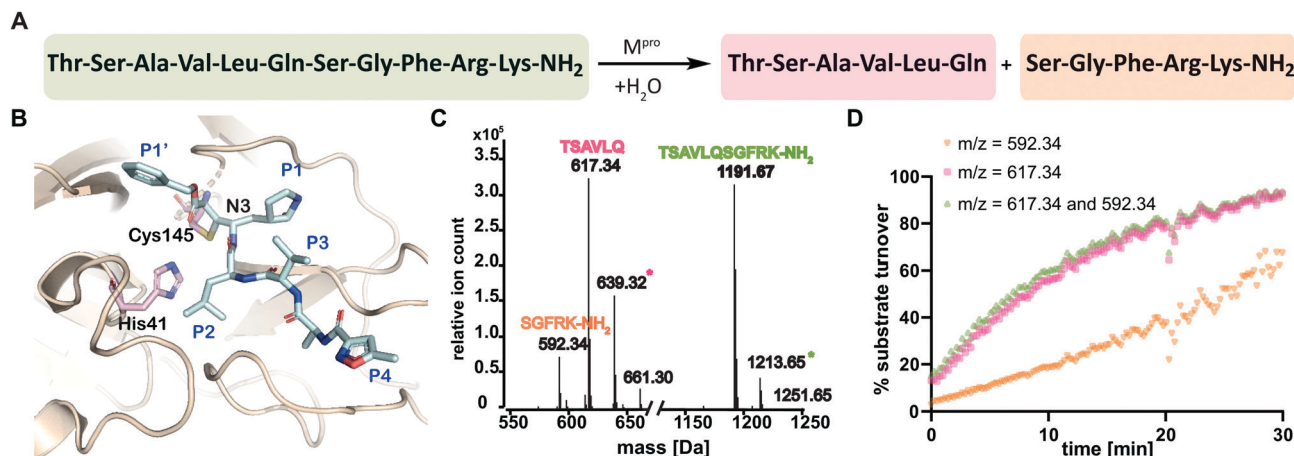
Fig. 1 SPE-MS assay monitoring \text{M}^{\text{Pro}} catalyzed cleavage of the TSAVLQ/SGFRK- \text{NH}_2 substrate. (A) \text{M}^{\text{Pro}} catalyzed hydrolysis of TSAVLQ/SGFRK- \text{NH}_2 . (B) View from a structure of Cys-145 linked \text{M}^{\text{Pro}} -N3 complex (PDB ID: 6LU7); 1 the Cys-His dyad is in pink; substrate binding sites are labelled in blue. (C) Deconvoluted mass spectrum of substrate/cleaved products after 10 minute incubation with \text{M}^{\text{Pro}} . Note, the C-terminal product was not efficiently retained by the SPE cartridge resulting in a low abundance compared to the N-terminal cleavage product. Sodium ion adducts (+23 Da) for the TSAVLQ product (639 Da) and substrate (1214 Da) are labelled with magenta and green asterisks, respectively. (D) % substrate turnover based on integration of the total abundance of cleaved products (TSAVLQ or SGFRK- \text{NH}_2 ) or the individual products. Conditions: 0.15 \mu\text{M} \text{M}^{\text{Pro}} , 2.0 \mu\text{M} TSAVLQ/SGFRK- \text{NH}_2 (1192 Da) (20 mM HEPES, pH 7.5, 50 mM NaCl).
