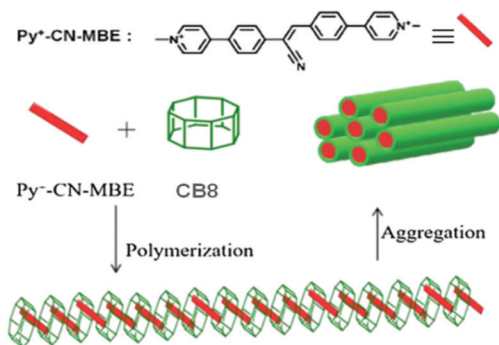
Scheme 20 Schematic representation of the Py + -CN-MBE-CB8 based polymer formation. The scheme has been reproduced from ref. 25 with permission from Wiley-VCH Verlag GmbH.
